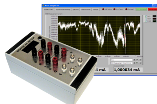
M100 Bridge mA-meter
